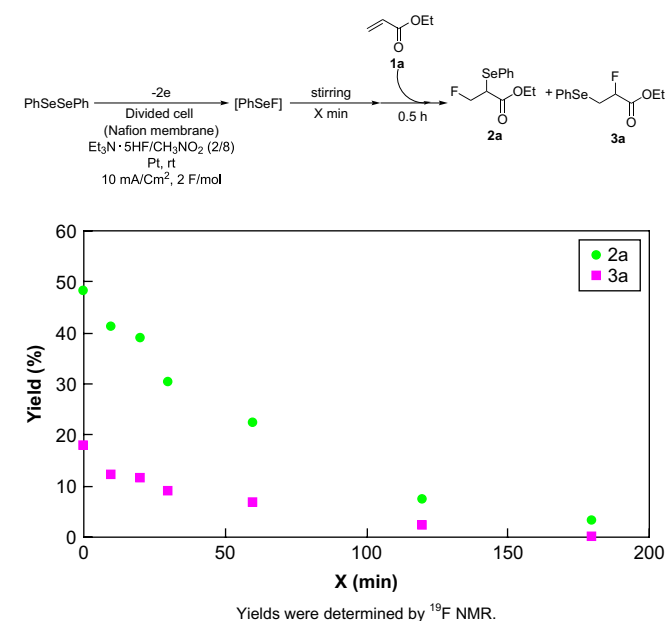
Figure 1. Relationships between yields ( 2a and 3a ) and initiation time of the reaction with 1a after electrolysis of (PhSe) 2 .
